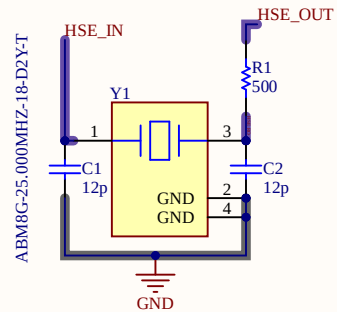
High Speed Oscillator 25MHz
