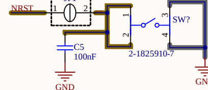
Reset Button
