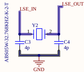
Low Speed Oscillator 32KHz
