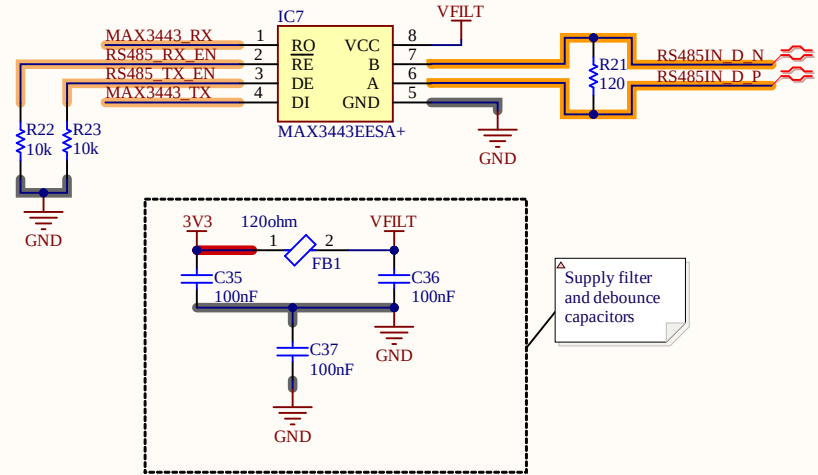
Breakout RS485
